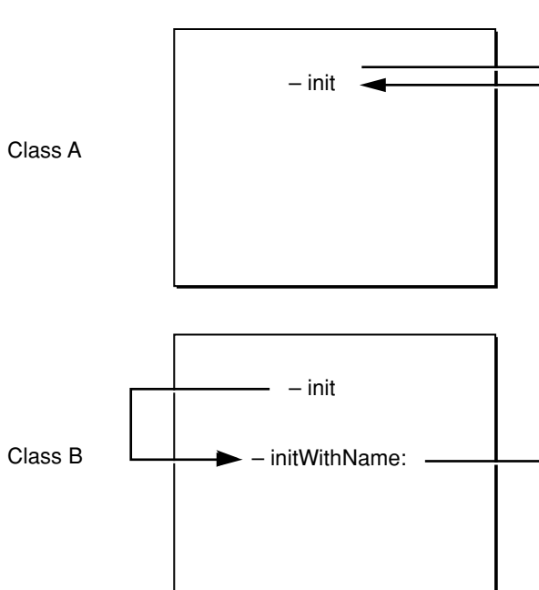
Figure 4-2 Covering an Inherited Initialization Model
