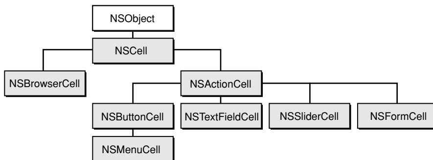
Figure 3-3 Inheritance hierarchy for NSCell
