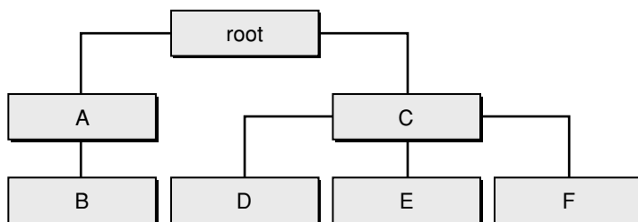
Figure 2-4 Inheritance Hierarchy
