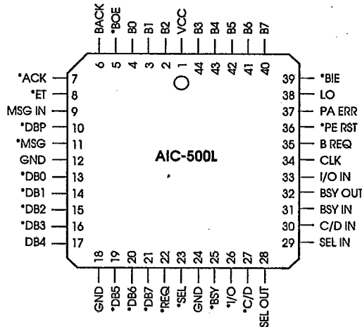
AIC-500 Quad PLCC Package
