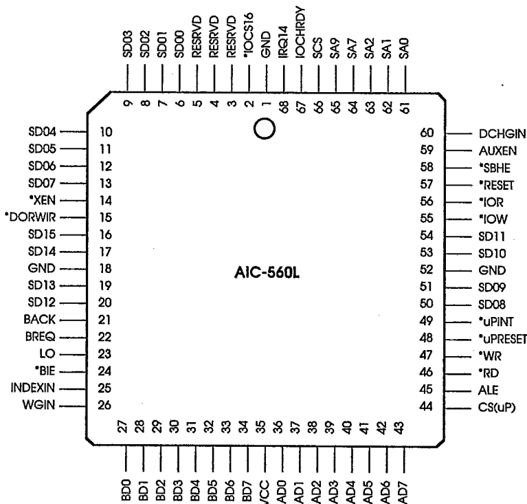
AIC-560 Quad PLCC Package
